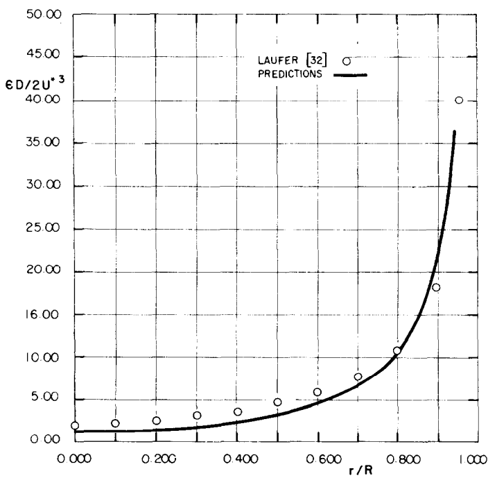
FIG. 4. Comparison of measured and predicted isothermal dissipation rate of turbulent kinetic energy, \epsilon , Re = 50,000 .
