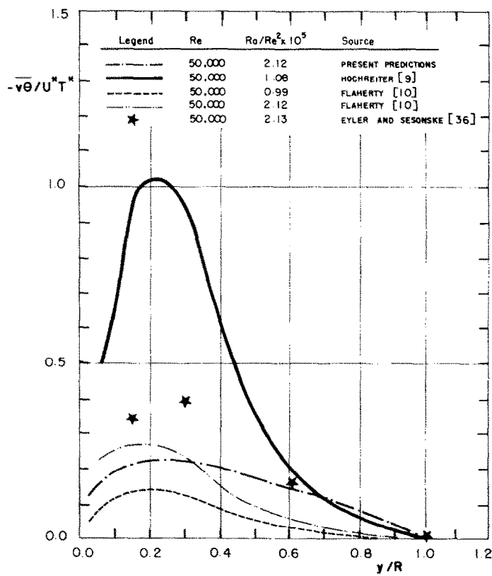
FIG. 14. Comparison of measured and predicted radial turbulent heat flux, \overline{v\theta} , Re = 50,000 .
