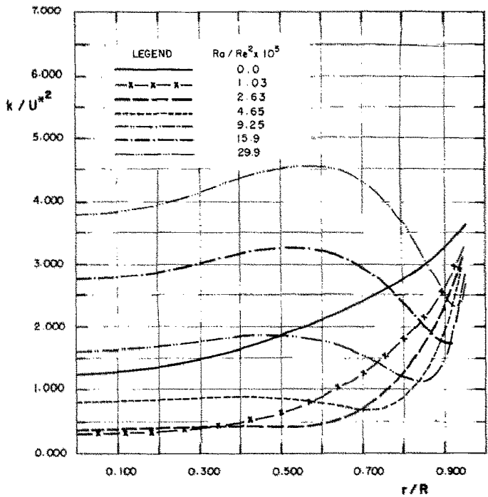
FIG. 9. Effect of heating on turbulent kinetic energy, k , Re = 30,000 .
