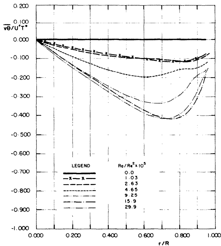
FIG. 15. Effect of heating on radial turbulent heat flux, \overline{v\theta} , Re = 30,000 .
